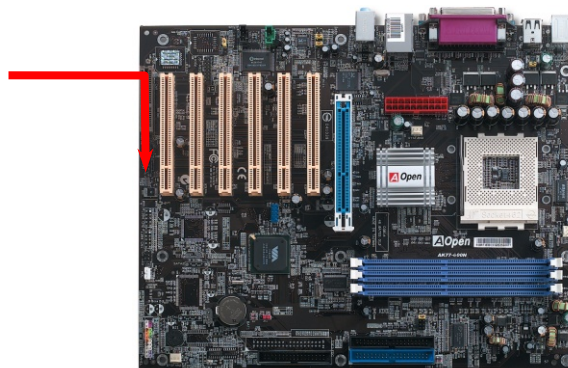
WOM Connector
